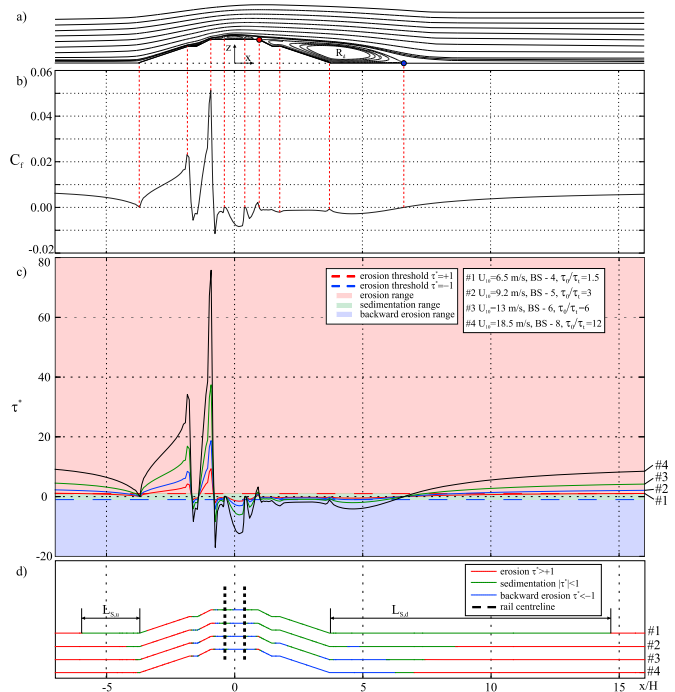
Fig. 8. Global flow features and potential sedimentation zones: a) reference flow topology; b) Skin friction coefficient; c) Shear stresses for different incoming reference velocities; d) Potential sedimentation, erosion and backward erosion zones.
