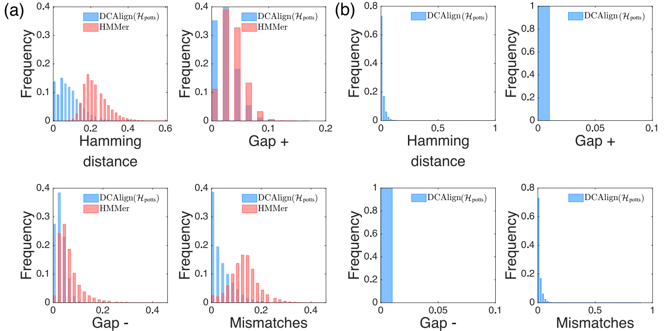
FIG. 6. Comparison between DCAAlign and HMMer for synthetic data. Panels (a) and (b) show the histograms of the normalized metrics (Hamming distance, \text{Gap}_+ , \text{Gap}_- , and Mismatches), respectively, in the case of conserved sites only, and of correlated pairwise columns only. Here, the reference is the ground truth and the target is the alignment of DCAAlign (blue) or HMMer (red). In panel (b), HMMer results are not shown because hmmsearch does not find any relevant hit.
