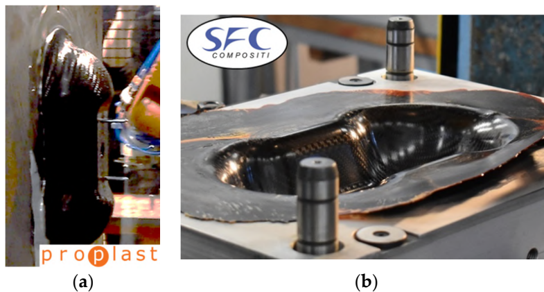
Figure 27. GF/PP and CF/PA66 Double Dome obtained by Horizontal Press (a), CF/EP-Angeloni and CF/EP-Solvay Double Dome obtained by Vertical Press (b).
