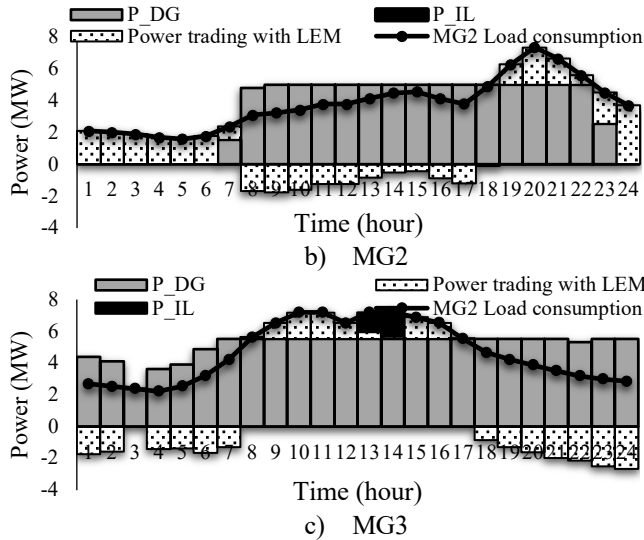
Fig. 9. Demand-supply Balance in each MG in Case II.
