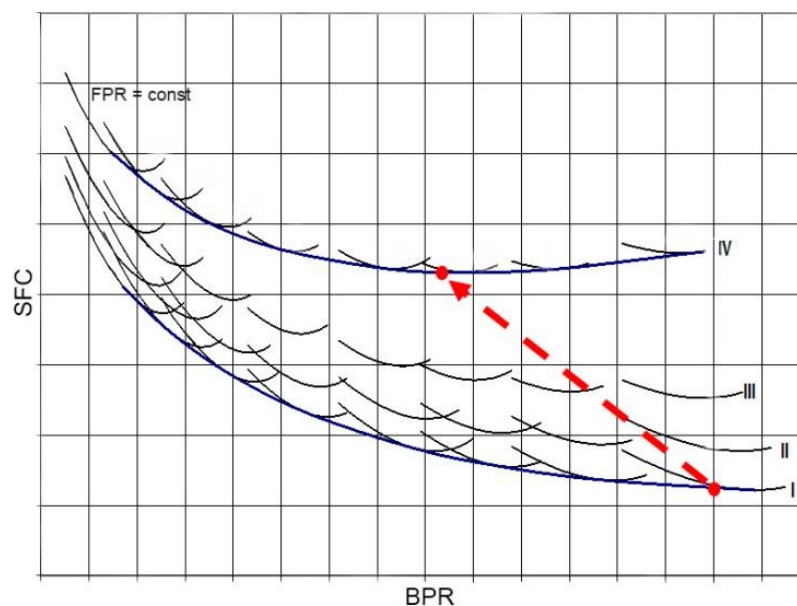
Figure 3. Dependences of uninstalled and installed cruise SFC on BPR at different FPR.
