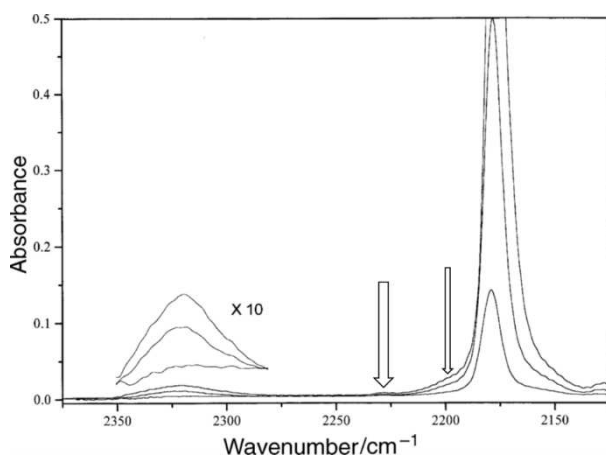
Figure 3. IR spectra of CO adsorbed on Na-ZSM-5. Arrows show combination bands between \nu(C-O) and FR modes.
