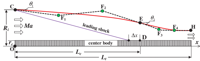
FIGURE 2. Parameterization of the basic flowfield.
