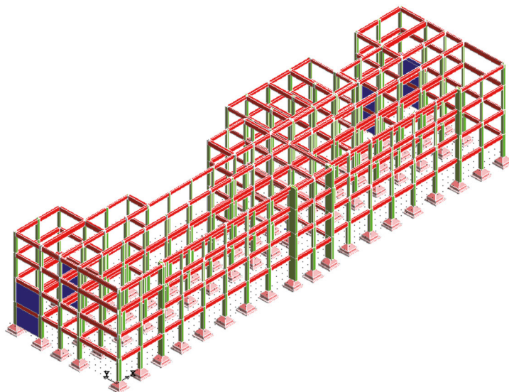
Fig. 3. FE model of the existing structure
