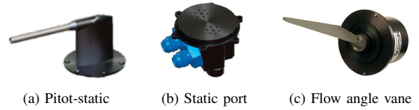
Fig. 2: Example of single function probe and vanes for pressure and flow angle measures
