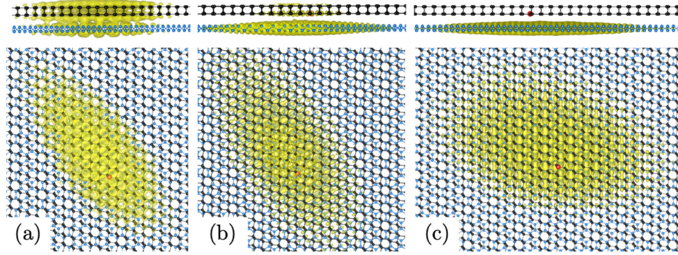
FIG. 4. Square modulus of the exciton wave function as a function of the electron position with fixed hole position. Side (upper panels) and top (lower panels) view of A_1 (a), B_1 (b) and B_2 (c). The hole is marked by the red sphere.
