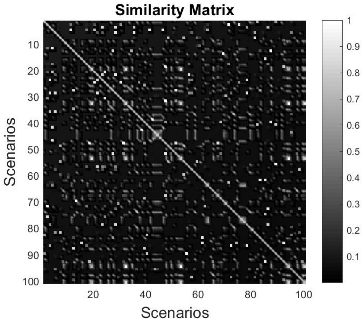
Figure 5 Similarity matrix \bar{W} containing the degree of similarity \mu_{ij} (2) between the N = 100 simulated transients: brighter areas mean higher similarity.
