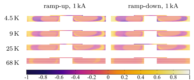
Figure 18. Current density distribution in the most inner turn of the upper deck, normalized with the critical current density at zero field and 4.5 K J_{\text{crit},0} = 138 \text{ kA mm}^{-2} . The distribution is given at 1 kA for both, the ramp-up and the ramp-down, for different temperatures.
