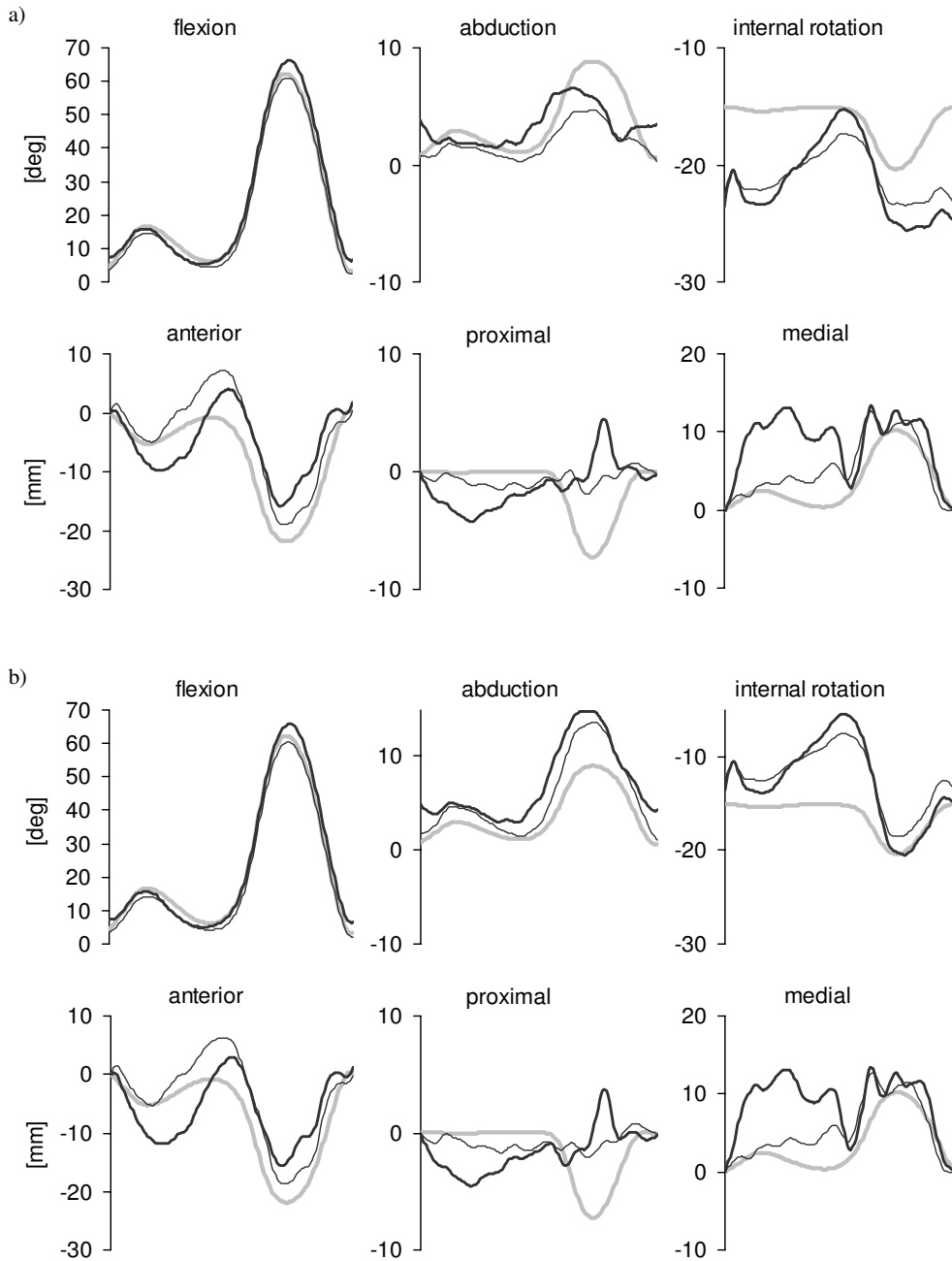
Patterns of the six knee kinematics components obtained after applying the selected pose estimators to the 12-marker cluster when instrumental errors and soft tissue artifacts were added to the marker nominal positions and the femur anatomical reference frame was made to rotate internally and externally as the effect of AL mislocations (a: +5 deg, b: -5 deg). See caption of Figure 4 for legend details. PCTa estimated patterns are not included.
