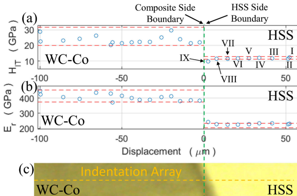
Figure 19. Indentation hardness (a) and reduced modulus (b) vs. displacement along the nIT array across a narrow (less than 10\ \mu\text{m} ) transitional layer. The red dashed lines show the ranges of indentation hardness and reduced modulus characteristics of the base materials, (c) is the optical microscopy image taken from the positioning system of the nano-indenter machine. The Roman numerals indicate the nine nano-indentation imprints on the HSS side, according to Figure 17. The green dashed line indicates the HSS/WC-Co interface. The green dashed lines indicate the composite and the HSS side boundaries of the transitional layer. The thickness of the transitional layer is less than the distance between two nano-indentations, thus both its boundaries lie on the same dashed line.
