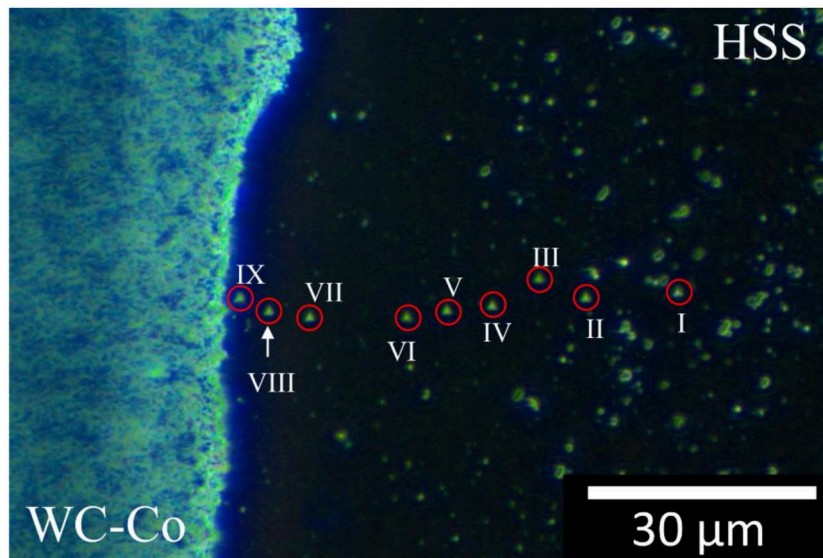
Figure 18. Dark Field Optical Microscopy image of an nIT linear profile across the weld-line. Here the transitional layer is wide, that is, about 50\ \mu\text{m} , as in Figure 9 (black arrow). The red circles and Roman numerals indicate nine (out of eleven) nano-indentation imprints on the HSS side; it should be pointed out that the profile continues on the WC-Co side, but it is not possible to discern the inherent nano-indentation imprints by means of OM.
