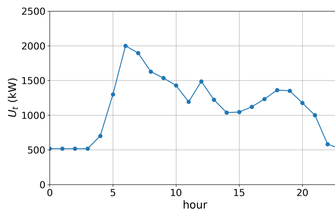
Figure 2. Heating power to be provided to the end-user over a 24 h period.
