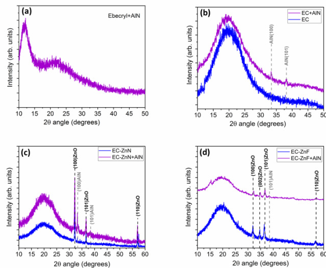
FIGURE 2. XRD spectra of all the analyzed samples: 2a) XRD spectrum of the pure acrylic matrix with AlN 600 nm-thick deposited; 2b) comparison of XRD spectra of the pure acrylic matrix (EC) with EC+AlN 600 nm-thick deposited; 2c) comparison of XRD spectra of the EC+nanoneedles with EC+nanoneedles+AlN; 2d) comparison of XRD spectra of the EC+nanoflowers with EC+nanoflowers+AlN.
