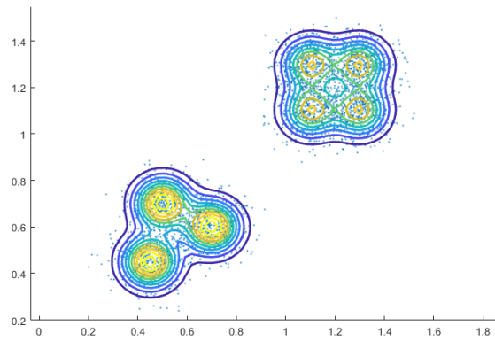
Fig. 11 GH-EXIN: Gaussian dataset. Data (blue points) and contours
