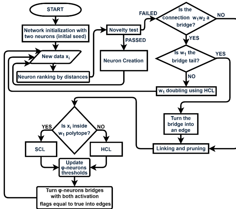
Fig. 1 G-EXIN flowchart
