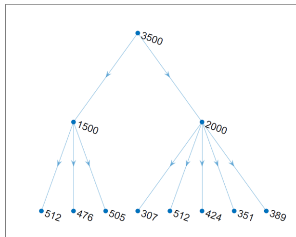
Fig. 14 GH-EXIN: Gaussian dataset, final tree and cardinality of nodes and leaves
