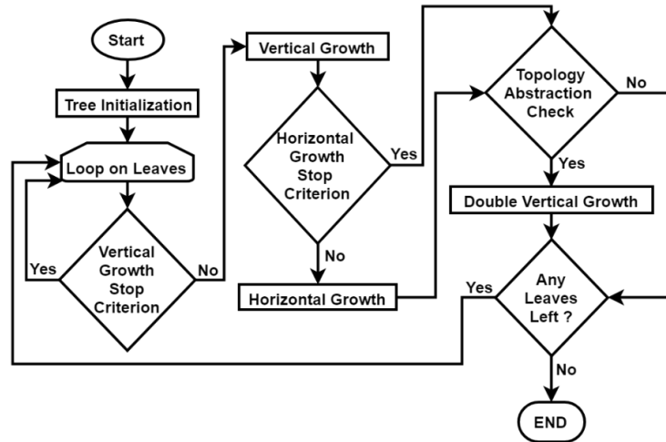
Fig. 3 GH-EXIN flowchart
