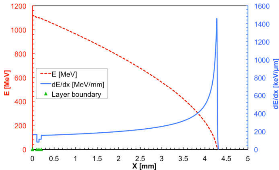
Figure 12. Energy loss profile in the telescope for an impinging ^{16}\text{O} ion with 70 MeV/amu kinetic energy.
