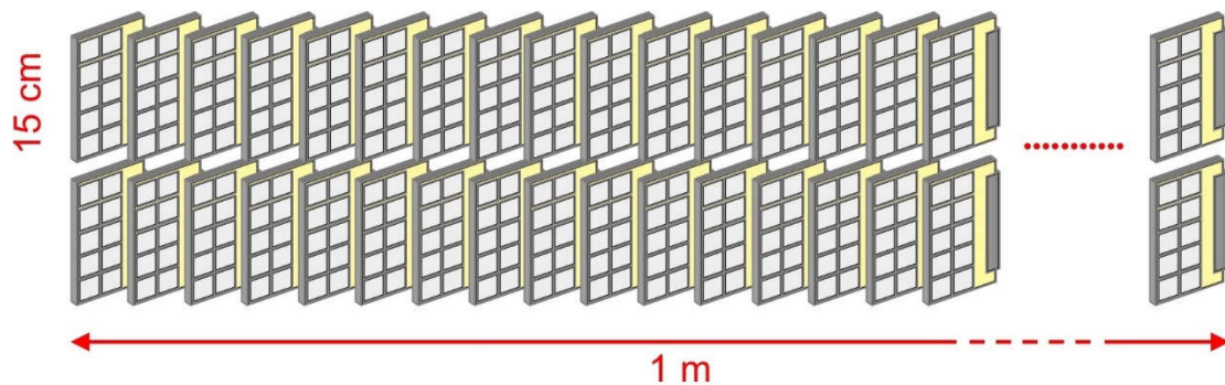
Figure 14. The full width of the Magnex focal plane (1 m), will be covered by 41 towers rotated by about 35^\circ with respect to the vertical axis to compensate the tilting angle of the focal plane with respect to the dipole magnet output.
