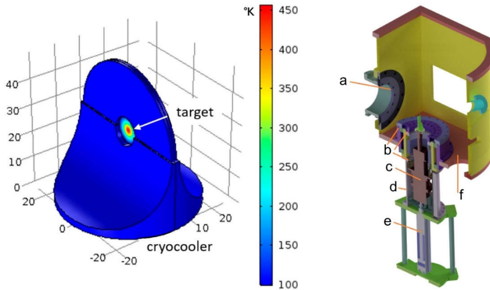
Figure 4. Left: Simulation of the temperature distribution on a ^{116}\text{Sn} target and its holder with a 50\ \mu\text{A} beam of ^{18}\text{O} at 15\ \text{MeV/amu} . The temperature does not exceed the fusion point. Right: 3D sketch of the target cryocooler in the scattering chamber. (a) connection flange to the forward beam pipe; (b) vacuum seal housing; (c) cryorefrigerator; (d) cylindrical guide for vertical motion; (e) vertical actuator; (f) chamber base platform.
