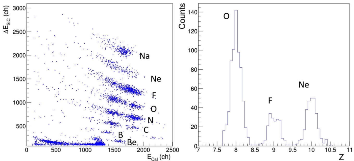
Figure 24. Left: \Delta E - E_r plot like where the atomic number of the ejectiles can be determined. Right: distribution of a few ejectiles close to oxygen as a function of their atomic number, following a linearization and projection procedure.
