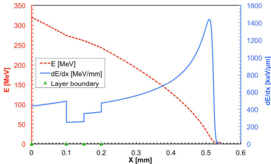
Figure 11. Energy loss profile in the telescope for an impinging ^{16}\text{O} ion with 20 MeV/amu kinetic energy.
