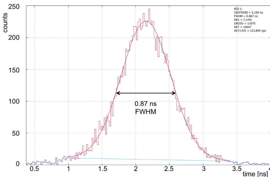
Figure 28. Coincidence time spectrum between two LaBr scintillators hit by back-to-back 511 keV gamma rays emitted by a ^{22}\text{Na} source. The FWHM resolution is well below 1 ns.
