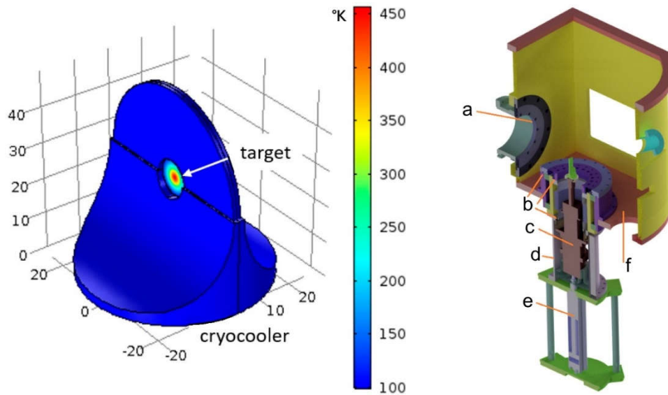
Figure 4. Left: Simulation of the temperature distribution on a ^{116}\text{Sn} target and its holder with a 50\ \mu\text{A} beam of ^{18}\text{O} at 15\ \text{MeV/amu} . The temperature does not exceed the fusion point. Right: 3D sketch of the target cryocooler in the scattering chamber. (a) connection flange to the forward beam pipe; (b) vacuum seal housing; (c) cryorefrigerator; (d) cylindrical guide for vertical motion; (e) vertical actuator; (f) chamber base platform.
