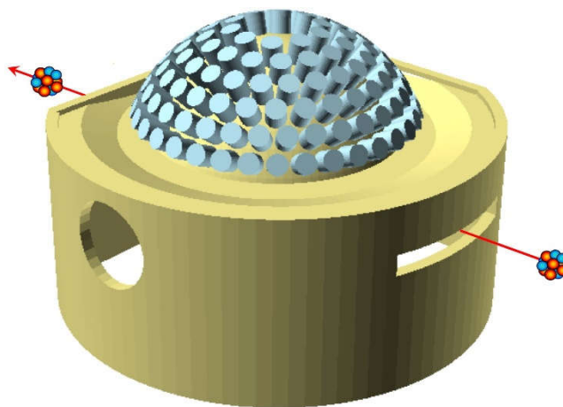
Figure 15. Sketch of the proposed configuration for the Gamma Detector Array (GDA). It consists of 139 \text{LaBr}_3(\text{Ce}) cylindrical scintillators, 38 mm diameter and 50 mm length, readout by means of photomultiplier tubes and arranged in six concentric rings pointing at the target at 25 cm distance and covering \approx 20\% of the total solid angle.
