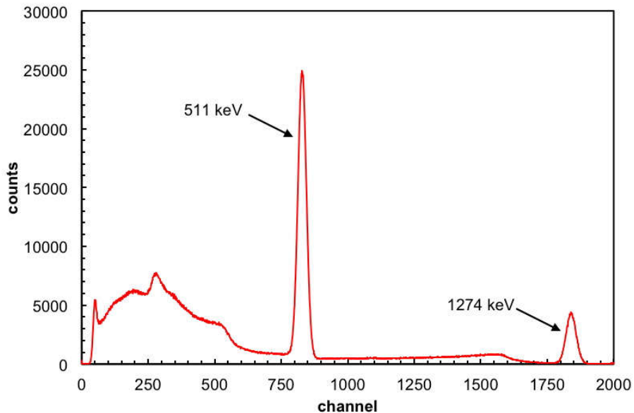
Figure 27. Energy spectrum of a ^{22}\text{Na} radioactive source obtained with a LaBr scintillator of the GDA detector. The peaks at 511 keV ( \beta^+ annihilation) and 1274 keV (direct gamma decay) respectively around channel 830 and 1840, are clearly visible, with FWHM resolution of 4% and 2%, respectively.
