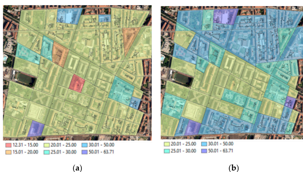
Figure 9. Solar Reflectance Index ( SRI ) (%) values of existing roof at block-of-building scale: (a) Before (b) and after high-reflectance strategy.
