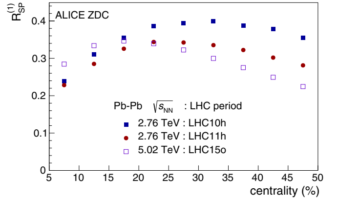
FIG. 1. The correction R_{SP}^{(1)} for finite resolution of the spectator plane angle \Psi_{SP} as a function of collision centrality for three data sets used in the analysis. Only statistical uncertainties, which are smaller than a symbol size, are shown.
