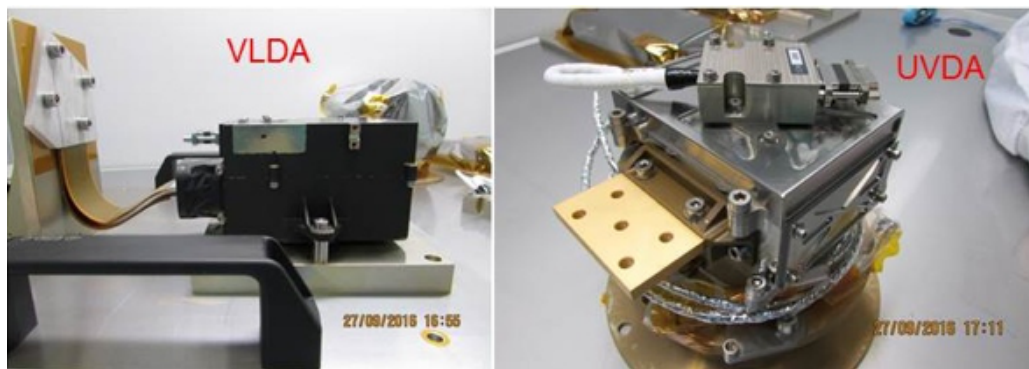
Fig. 13. Detector units at delivery at the Optical Payload Systems facility at ALTEC in Turin. The two cameras, VLDA, and UVDA are mounted face down on the transport plates.
