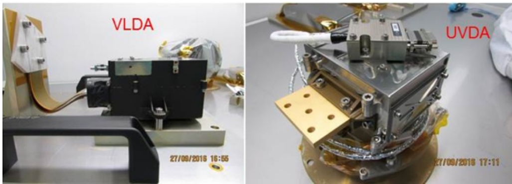
Fig. 13. Detector units at delivery at the Optical Payload Systems facility at ALTEC in Turin. The two cameras, VLDA, and UVDA are mounted face down on the transport plates.
