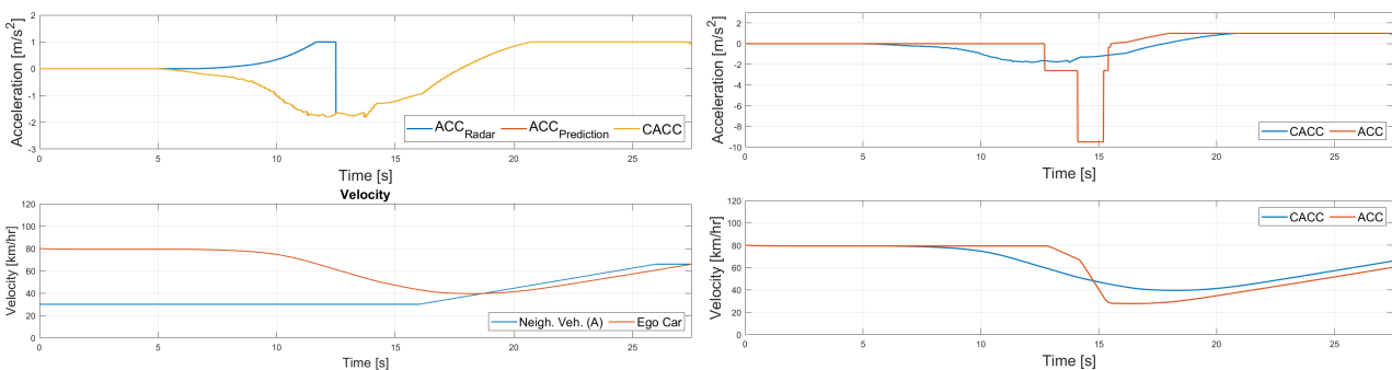
Fig. 5. Scenario2. Left: Ego car acceleration (top) and speed trend (bottom). Right: acceleration (top) and speed (bottom) under ACC and CACC.
