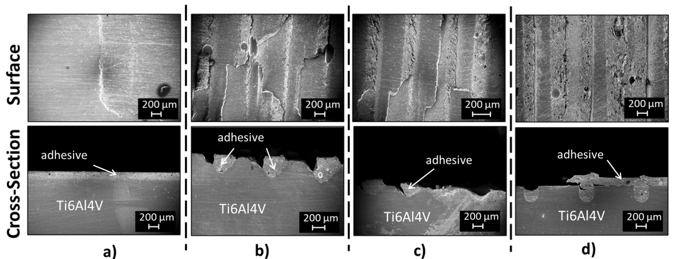
Figure 8 Joint fracture analysis at higher magnification: top view and cross-sectional micrographs (a) Unmodified surface, (b) Semi-overlapped V-shaped micro-slot surface, (c) Interlocked semi-circle shaped micro-slot surface, (d) Semi-overlapped U-shaped micro-slot surface; all the tested samples were oriented perpendicular to the load.
