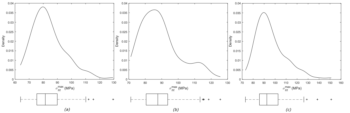
Figure 20: Fitting of the probability density function of \sigma_{zz}^{max} with applied \epsilon_{zz} (a) RVE-1 and VD-1, (b) RVE-2 and VD-1, (c) RVE-2 and VD-2, void content 5%
