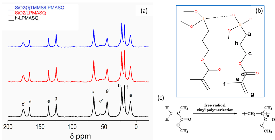
Figure 8. (a) ^{13}\text{C} CPMAS spectra of h-LPMASQ (black line), \text{SiO}_2/\text{LPMASQ} (red line) and \text{SiO}_2@\text{TMMS}/\text{LPMASQ} (blue line). The LPMASQ structure with C labeling and the polymerization scheme [68] are shown in figures (b) and (c), respectively.
