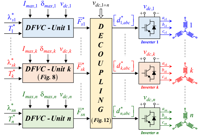
Fig. 5. Modular DFVC scheme for multi-three-phase IM drives.
