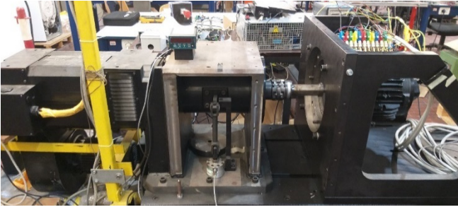
Fig. 15. View of the machine under test (right) and driving machine (left).
