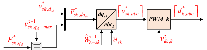
Fig. 18. Conventional MS-based DFVC scheme: the output of the k -unit torque controller is considered as the q_{sk} -axis reference voltage of the unit k .
