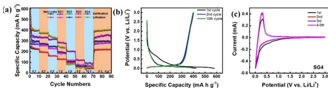
Figure 4. (a) Galvanostatic lithiation/delithiation curves, (b) Lithiation/delithiation voltage profiles and (c) cyclic voltammety curves of semi-coke derived graphene anode measured at a scanning rate of 0.5 \text{ mV s}^{-1} . Reproduced, adapted and reprinted with permission from Reference [77].
