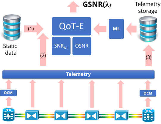
Fig. 1 QoT-E module predicting the GSRN(\lambda) using static data from factory characterizations of network elements (1), data form telemetry (2) or stored data from telemetry feeding a ML module (3).
