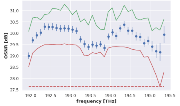
Fig. 3 Blue dots: mean value of the OSNR measured on each channel; errorbars: standard deviations. In green and red, respectively, the maximum and the minimum for each channel. The dashed line indicates the overall minimum OSNR.
