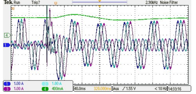
Fig. 20. Oscilloscope screenshot of phase currents (phases a1, a2, a3 ; 1 A on oscilloscope = 0.25 A of real current) and electromagnetic torque measured with torque meter (400 mA = 0.5 Nm of real torque). Waveforms filtered with a 2.9 kHz filter.
