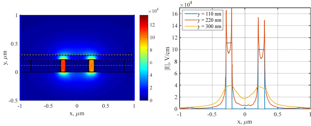
Fig. 6. Left: RF electric field map simulated with the QS solver. The black lines are used to indicate the device geometry, to assist the direct comparison with Fig. 1(right). The three dashed horizontal lines intersect the slot center (blue, y = 110 nm), the slot top (red, y = 220 nm), the end of the NLO material (orange, y = 300 nm). Right: cuts of the maps on the left (the small oscillations result from the interpolation of the different meshes, necessary to perform the multiphysics coupling (3)). The three cuts correspond to the horizontal lines intersecting the slot center (blue, y = 110 nm), the slot top (red, y = 220 nm), the end of the NLO material (orange, y = 300 nm).
