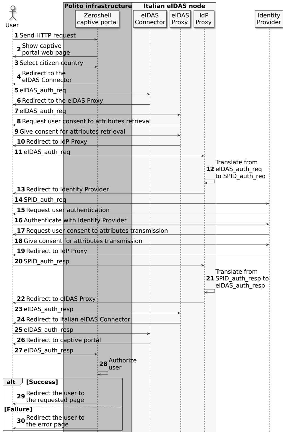
Figure 3: Authentication sequence diagram for Wi-Fi access for a citizen with an Italian SPID credential, by exploiting an eIDAS-enabled Zeroshell captive portal.
