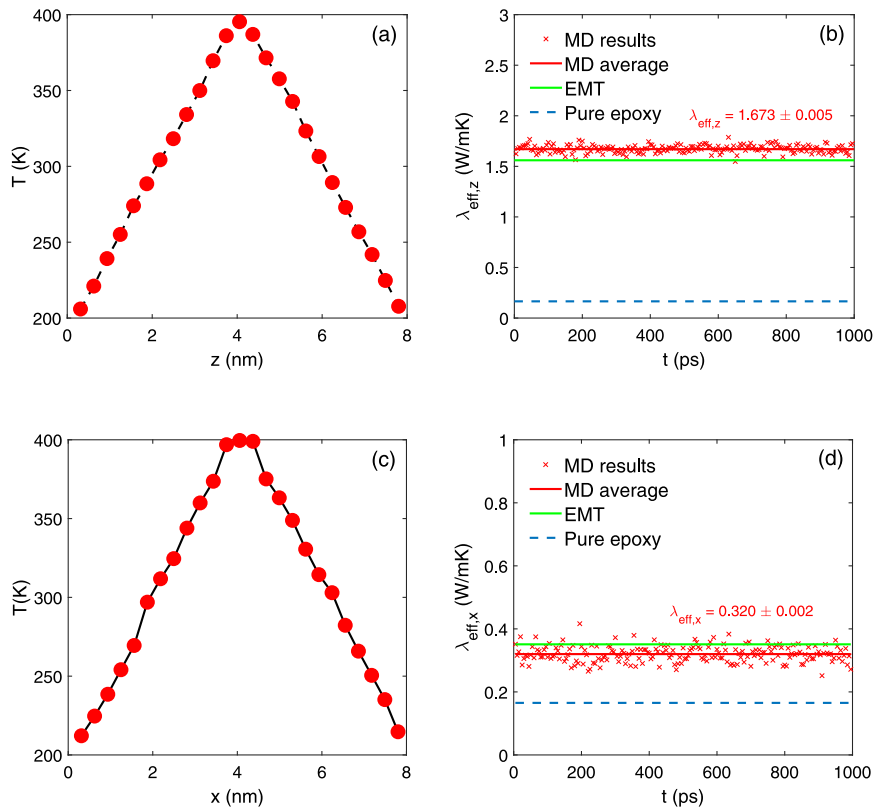
Fig. 11. (a) Temperature profile and (b) effective thermal conductivity along the main axis of the CNT (z direction) for the epoxy-based composite containing five nanotubes. (c) Temperature profile and (d) effective thermal conductivity perpendicular to the main axis of the CNT (x direction) for the epoxy-based composite containing five nanotubes. Red dots and solid lines represent MD results, green solid lines predictions by the EMT-based model, blue dashed lines MD result for pure epoxy.
