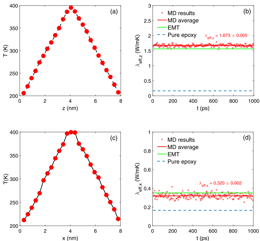
Fig. 11. (a) Temperature profile and (b) effective thermal conductivity along the main axis of the CNT (z direction) for the epoxy-based composite containing five nanotubes. (c) Temperature profile and (d) effective thermal conductivity perpendicular to the main axis of the CNT (x direction) for the epoxy-based composite containing five nanotubes. Red dots and solid lines represent MD results, green solid lines predictions by the EMT-based model, blue dashed lines MD result for pure epoxy.
