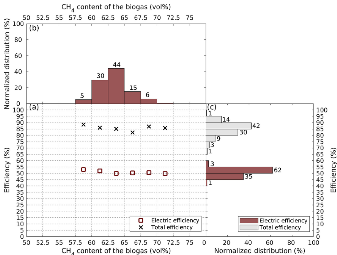
Fig. 4. Electric and total efficiencies of both Convion C50 systems as function of the CH 4 content of the biogas and corresponding normalized distributions. a) Electric (red squares) and total (black crosses) efficiency mean values for CH 4 content of the biogas segments during stable operation. Segments are represented by the vertical dashed lines. b) Normalized distribution of the CH 4 content of the biogas. c) Normalized distribution of the electric and total efficiencies. Combined standard uncertainties were around 3% for the electric and around 6% for the total efficiency. (For interpretation of the references to colour in this figure legend, the reader is referred to the Web version of this article.)
