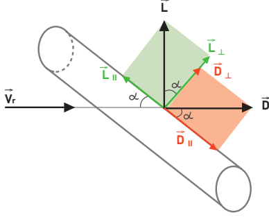
Fig. 5: Cylindrical cable segment invested by the wind
