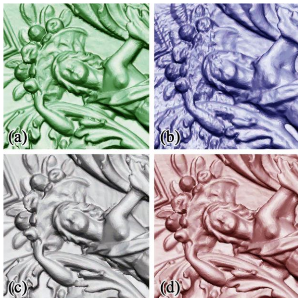
Figure 4. Particular of the meshes of the vault generated from the four datasets. (a) Faro Focus3D X 330, (b) Leica BLK360, (c) Leica RTC360, (d) Riegl VZ-400i.
