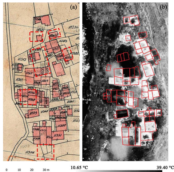
Figure 15. (a) Rabbini Cadastre and the investigated areas (red dashed polygons) detected on the thermal orthomosaic. (b) Overlay between the thermal orthomosaic and the shapes of the buildings (red polygons) reported in Rabbini Cadastre.
