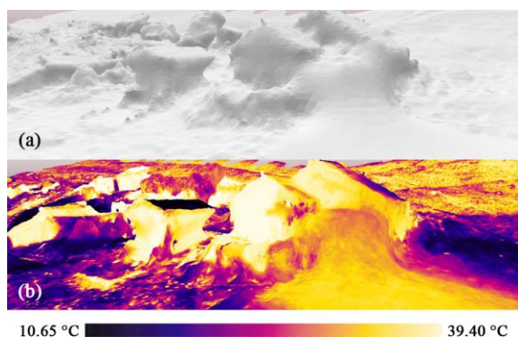
Figure 11. (a) Mesh triangulated from thermal dataset and (b) Texturized mesh (thermal data, IRON palette).
