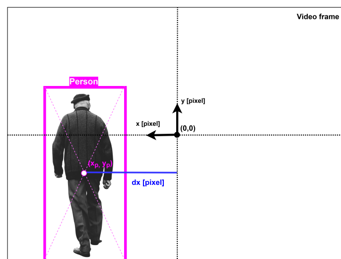
Figure 3. The RGB frame of the camera showing how the dx value, adopted in the computation of the angular velocity, is obtained. This value is equal to the horizontal coordinate of the center of the bounding box detecting the person in the frame.
