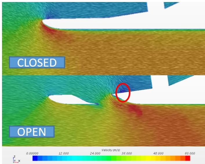
Fig. 8. Velocity distribution for high downforce mode (up) and low drag mode (down) splitter
