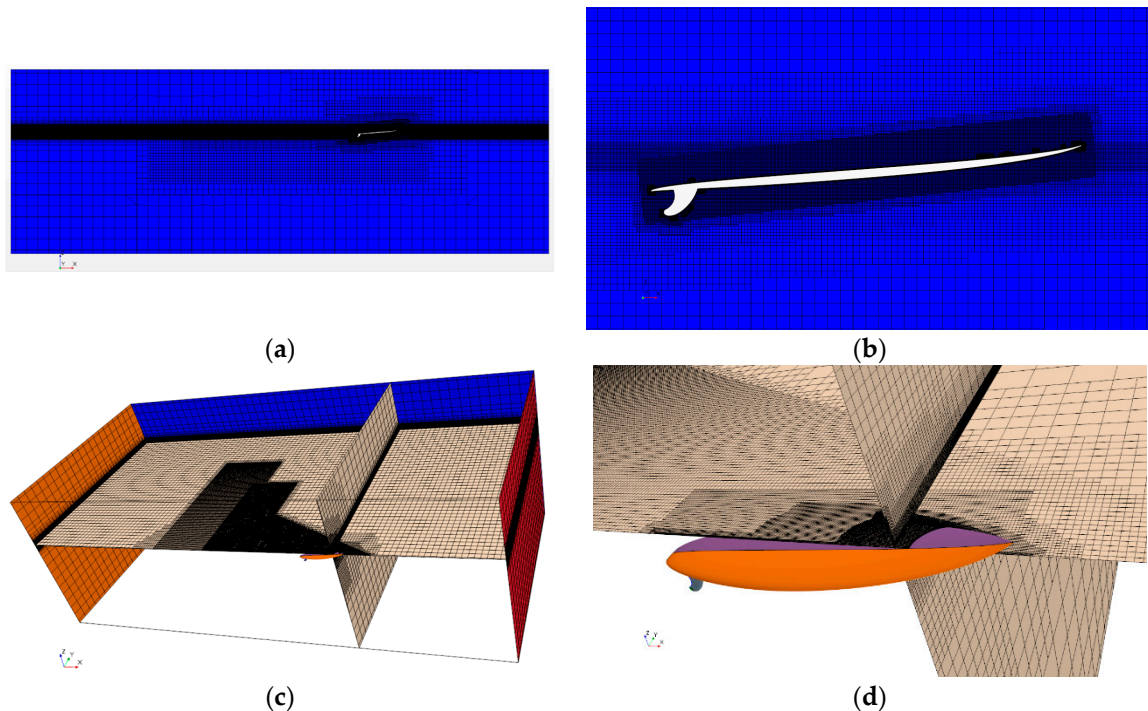
Figure 2. The computational mesh; (a) complete view at the symmetry plane; (b) zoomed view at the symmetry plane near the surfboard; (c) complete view of the computational domain; (d) mesh details near the surfboard.
