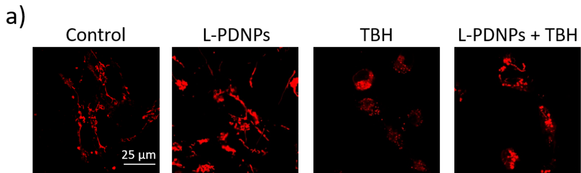
Figure 6. Analysis of mitochondrial morphology and membrane potential. a) Representative images of mitochondria in different experimental conditions (mitochondria in red, stained with TMRM). b) Median values of mitochondria roundness ( \rho ) in the same experimental conditions ( n = 3 , * p < 0.001 ). c) Mitochondria classification in sub-groups on the basis of the \rho values. d) Trend of mitochondrial membrane potential ( \Delta\Psi_m , based on fluorescence analysis). O: addition of 6 \mu\text{M} oligomycin ( n = 3 ).
