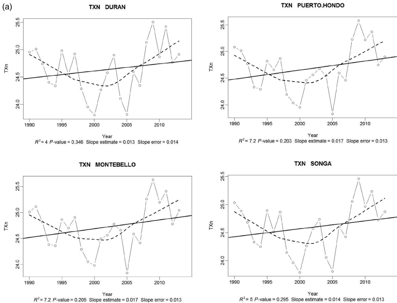
FIGURE 5 Outputs of the indices: (a) lowest maximum temperature (TXn); (b) mean maximum temperature (TmaxMean); and (c) daily temperature range (DTR) for each meteorological station. Reproduced is a curve representing the annually temporal evolution of the index, with the continuous line showing the estimation trend and the dotted line the locally weighted linear interpolation (locally weighted regression—LWR)
