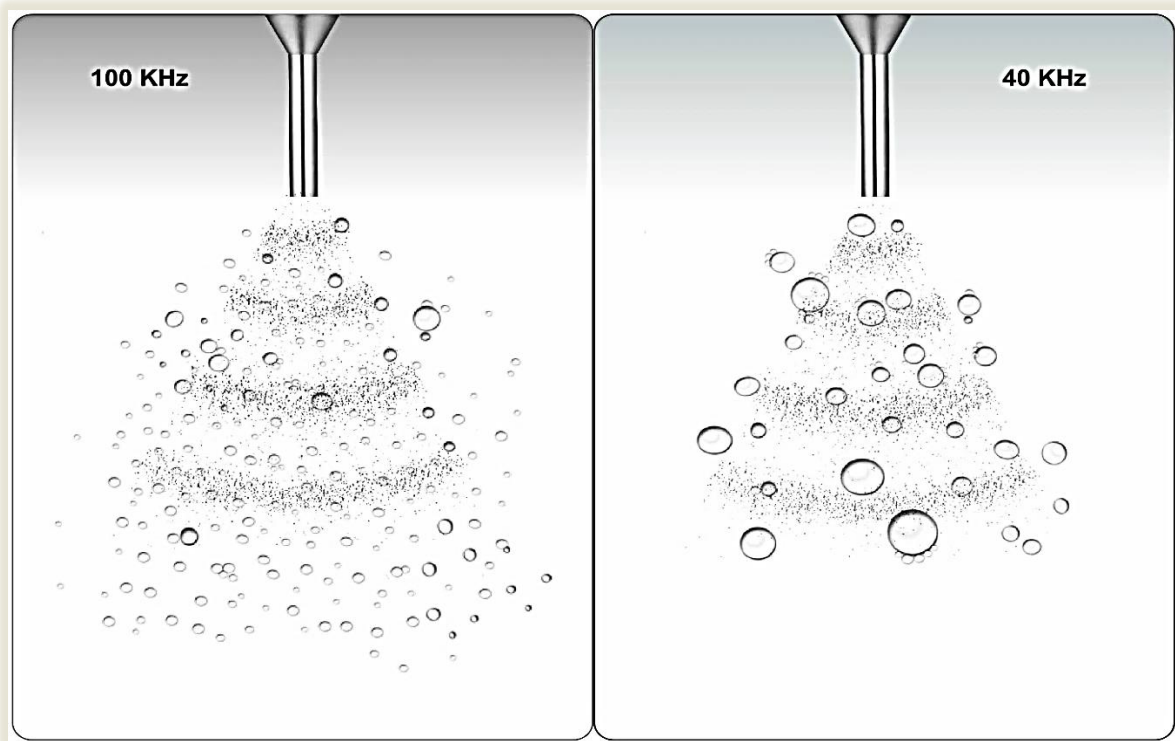
298 299 Fig. 5. The effect of implemented frequency on the size and population of the generated micro- 300 bubbles.
