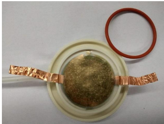
Fig. 7. Piezoelectric PVDF membrane sitting in the membrane cell. The membrane was sandwiched between two Au plates and the coating of each side was connected to a conductive copper tape respectively, [176].
