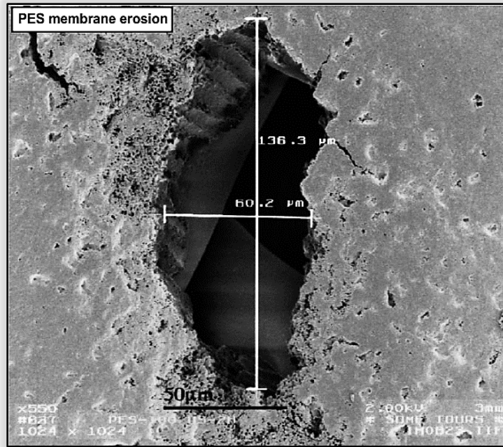
Fig. 6. Microscopic images of the highly damaged area of the PES membrane irradiated by ultrasonic waves; at a magnification of 550 [167].
