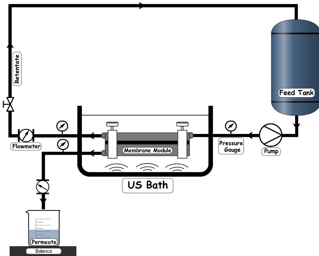
281 Fig. 3. Schematic of a simple ultrasonic bath used for membrane cleaning [101].
