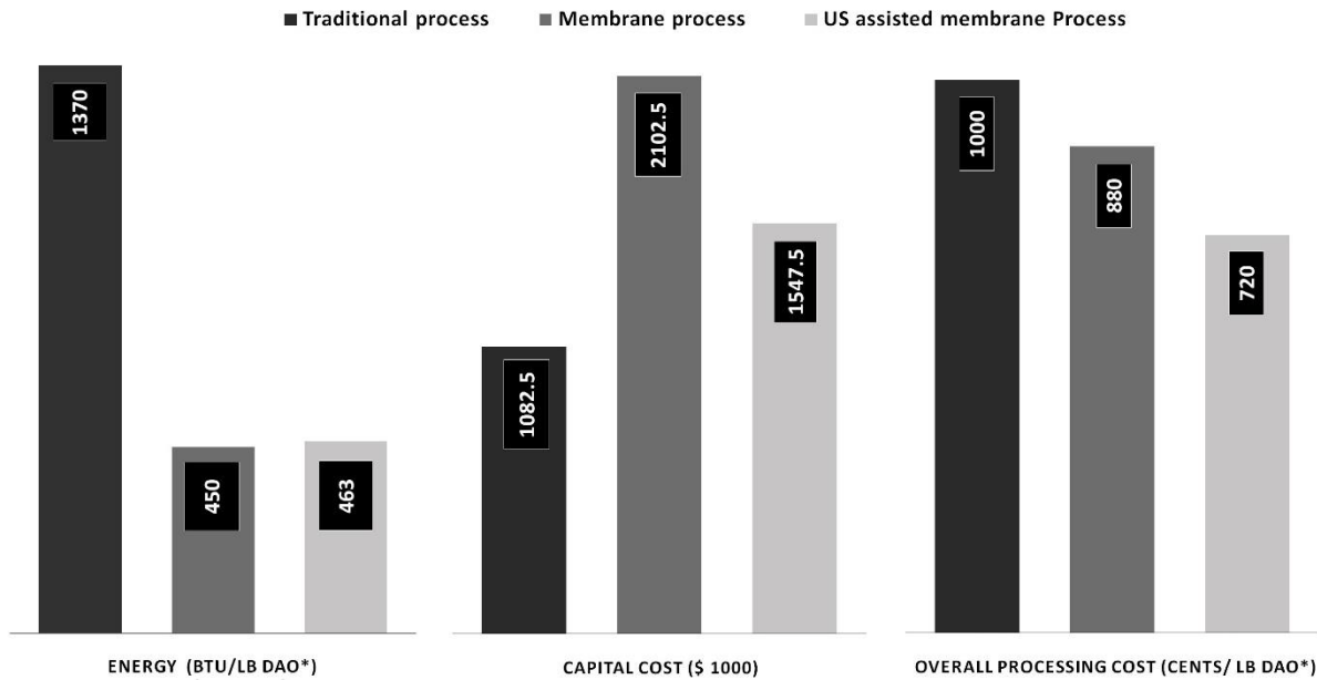
Fig. 8. Comparison of economic and energy advantages of piezoelectric membrane technology for solvent recovery in deasphalting operations [153].
