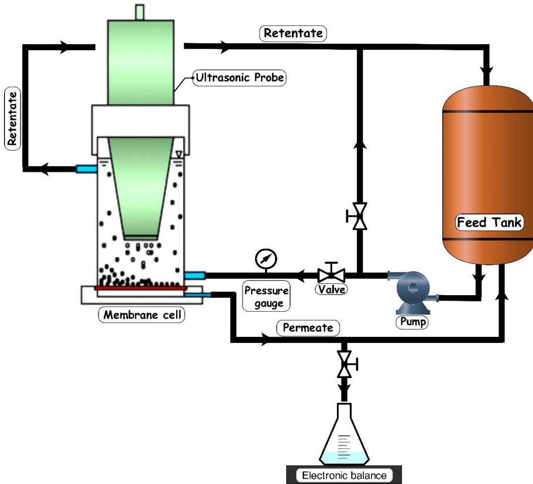
285 Fig. 4. Diagram of a membrane filtration system assisted with an ultrasonicator (homogenizer)
