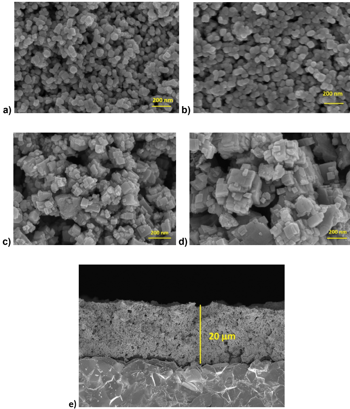
Fig. 5. FESEM micrographs of sensors (150 kx): SA- \text{In}_2\text{O}_3 (a), SA-W- \text{In}_2\text{O}_3 (b), HT- \text{In}_2\text{O}_3 (c), HT-W- \text{In}_2\text{O}_3 (d) and an image in cross-section of the sensitive layer (e).
