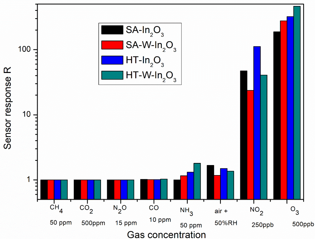
Fig. 15. Cross-sensitivity measurements for SA-In 2 O 3 , SA-W-In 2 O 3 , HT-In 2 O 3 and HT-W-In 2 O 3 sensor at 100°C.
