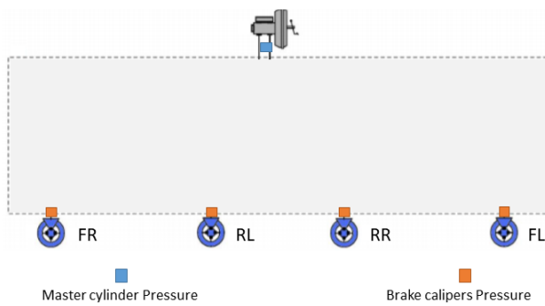
Figure 6: Schematic of braking system instrumentation
