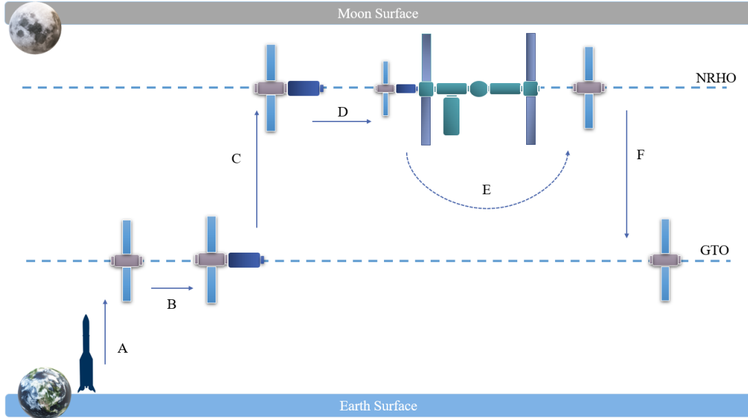
Figure 1: Design Reference Mission.
