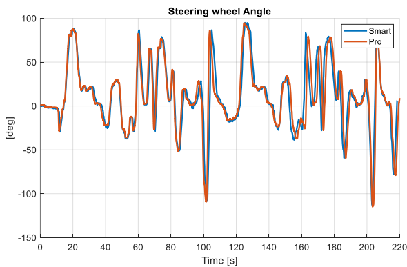
Figure 14 – Experimental validation: steering wheel angle during a lap on the handling test track.
