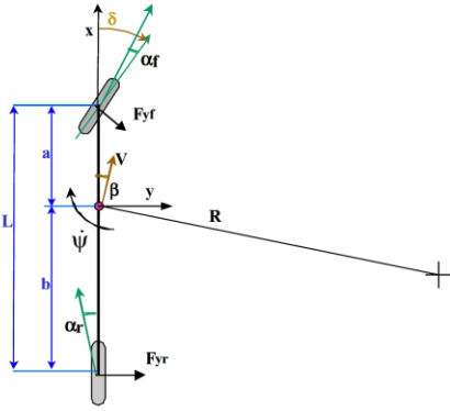
Figure 7. Single-track model scheme.
