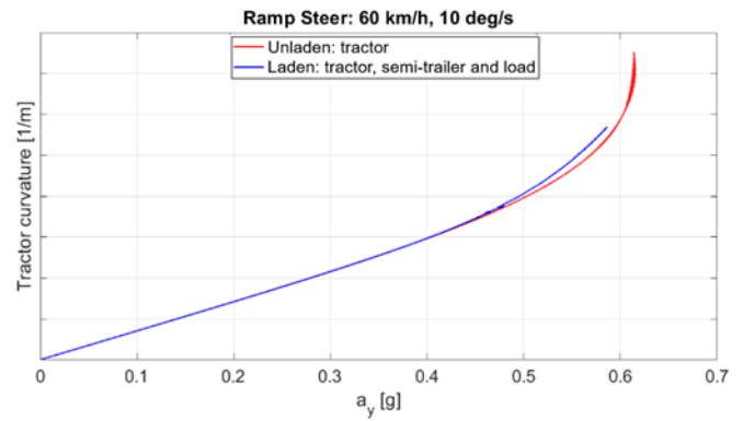
Figure 9. Ramp steer: Tractor curvature
