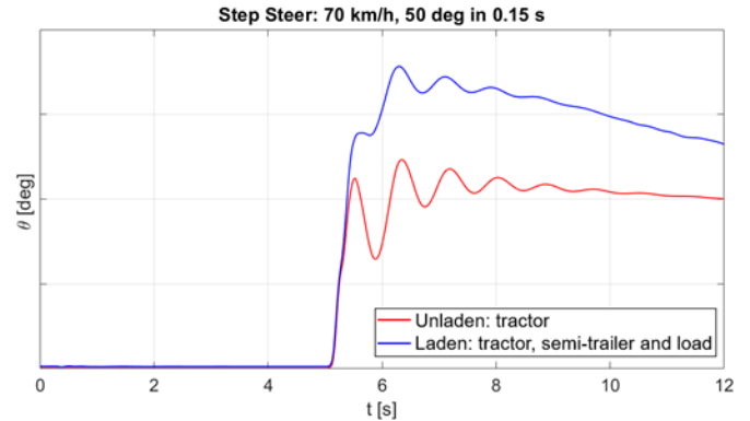
Figure 14. Step steer: Roll angle vs time
