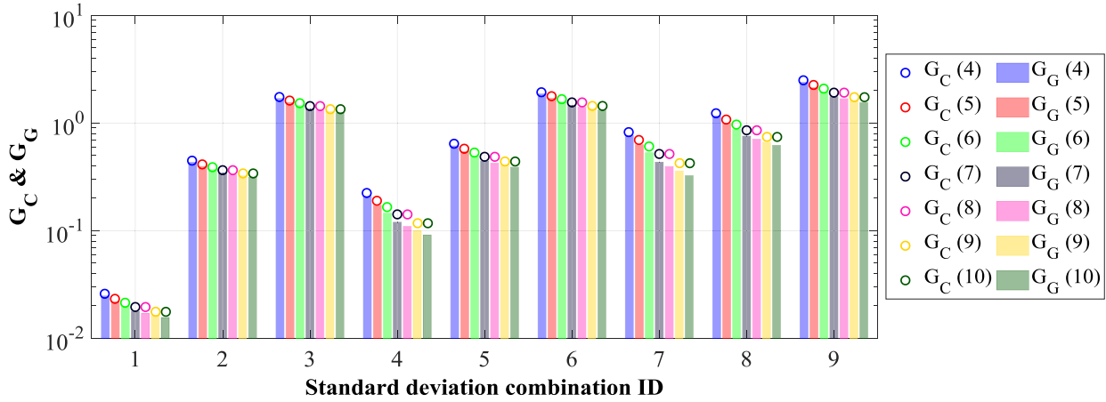
38 Fig. 7. Comparison of G_C and G_G in case of cantilever beam for all standard deviation combinations (number 39 in parenthesis of G_C and G_G denote the number of sensors).
