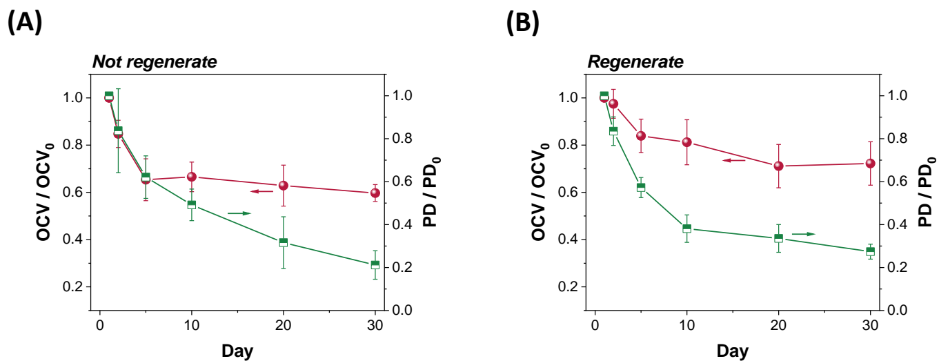
Figure S14. Long term stability of the membrane-free EFC. Relative voltage ( OCV/OCV_0 ) measured at open circuit conditions and relative power ( PD/DP_0 ) of the EFC fueled by 1 mM of glucose in PBS. (A) The enzyme is adsorbed on the anode at day 0 and kept as is until day 30, (B) the enzyme is replenished before each measurement.
