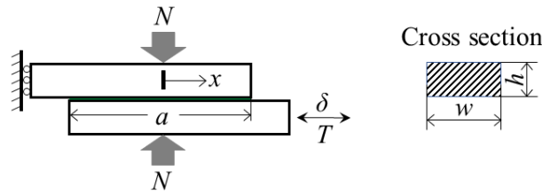
325 Fig. 8. Lap joint plates model and cross section of the plate
